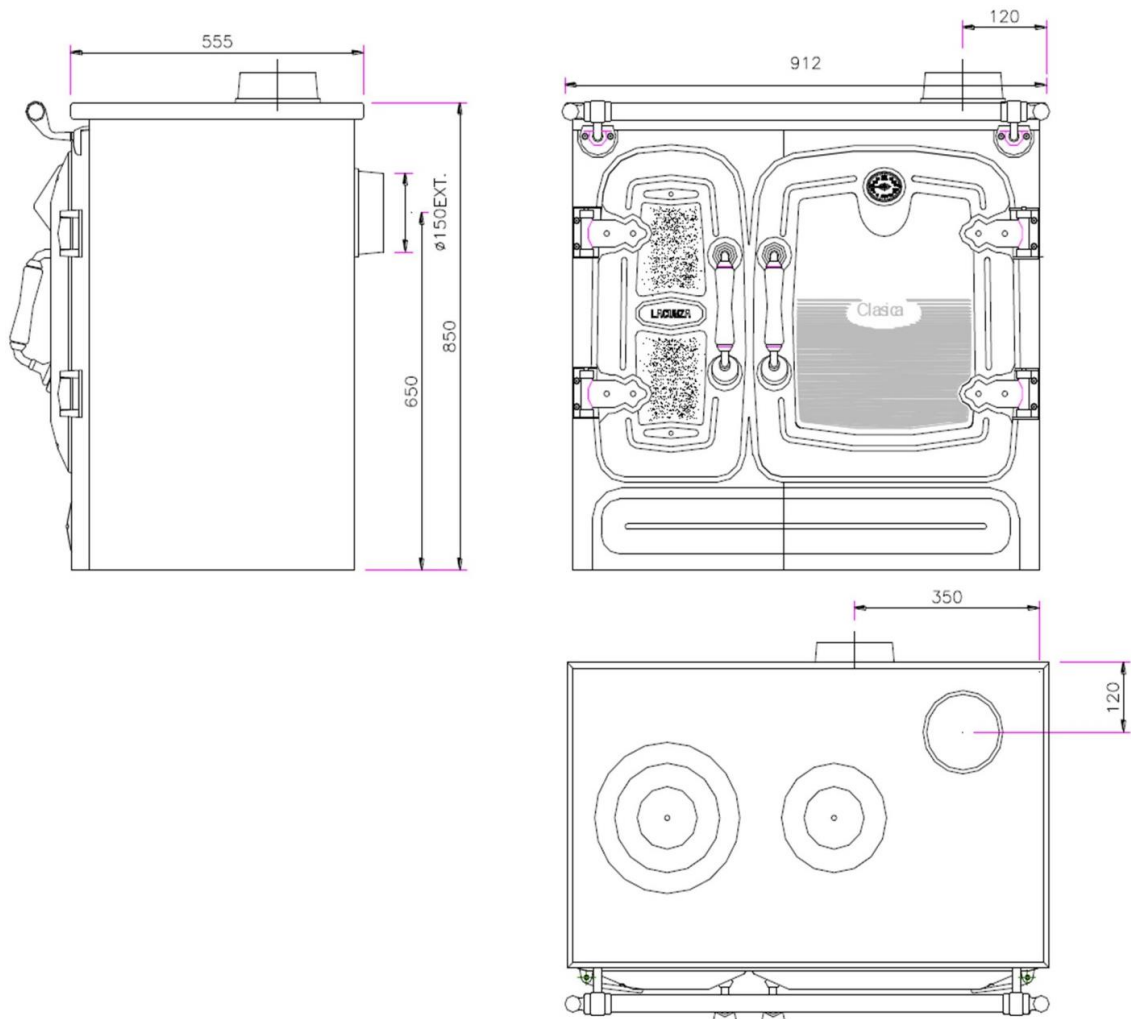
Figure No.2 - Dimensions of the Clásica 7T appliance in mm
