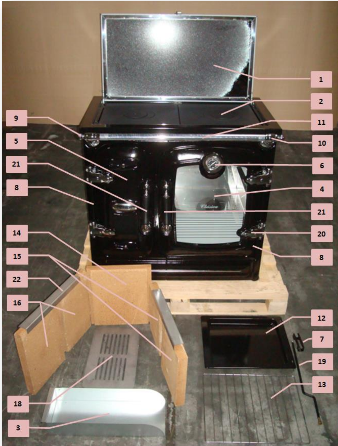
Figure No.18 - Basic breakdowns
