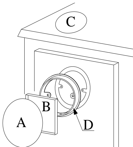
Figure No.6 - Diagram for rear flue socket
